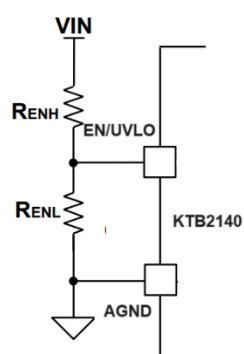
Figure 2. Configuring the Input UVLO Threshold through EN/UVLO Pin
