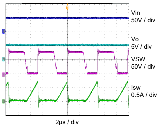
Enable Startup (24V IN , 5V O , I O = 3A)
