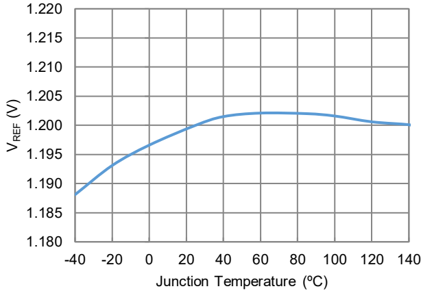
V_{REF} Temperature Regulation
