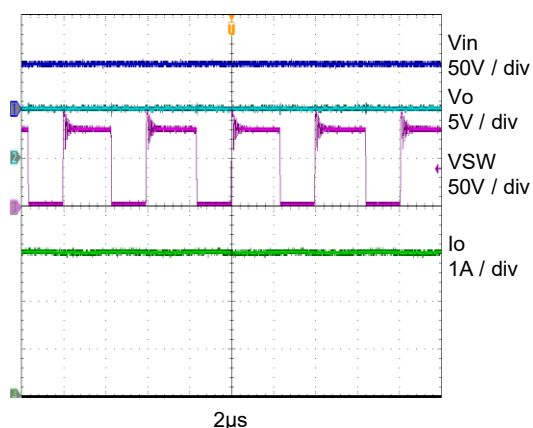
Stable Working at DCM (24V IN , 5V O , I O = 1A)
