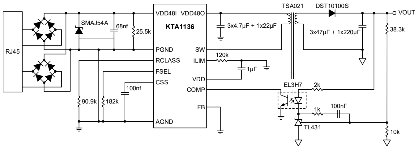
Figure 3. Flyback Application with Secondary Side Regulation
