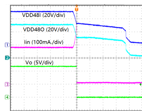
Shutdown by PSE at 1A Load
