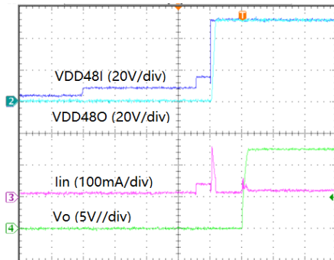
Startup with PSE Input at 0A Load
