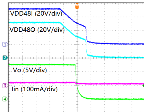
Shutdown by PSE at 0A Load
