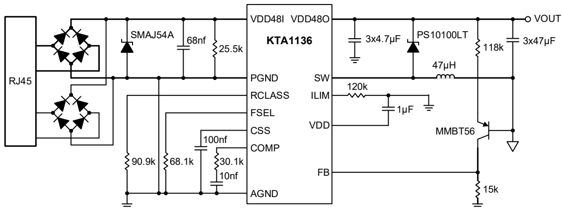
Figure 4. Simplified Buck Application
