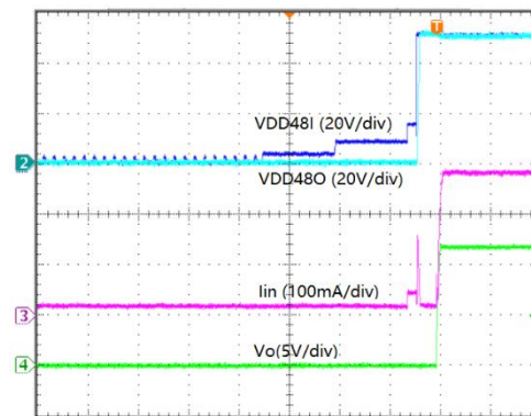
Startup with PSE Input at 1A Load
